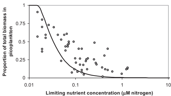
Fig. 2. Percentage of total biomass in the picoplankton size fraction ( <2 \mu\text{m} in diameter) as a function of nutrient availability ( \mu\text{M} nitrogen) for a dilution rate ( D , \text{h}^{-1} ) of 10^{-2} predicted by the physiological model and compared with field data of microbial size spectra compiled by Chisholm (1992). Total biomass is calculated assuming total biovolume is linearly proportional to carbon. Field data compiled by Chisholm (1992) was compared with the model predictions by converting \mu\text{g Chl-}a \text{ l}^{-1} to \mu\text{M} nitrogen using \text{C Chl}^{-1} (\text{wt/wt}) = 10 and assuming C:N in biomass is in Redfield proportions.
